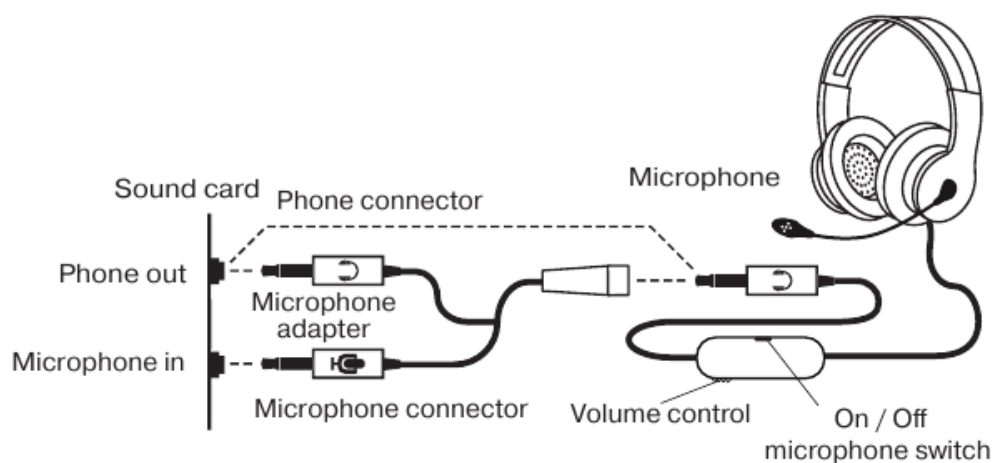
Fig. 1. Connection diagram
