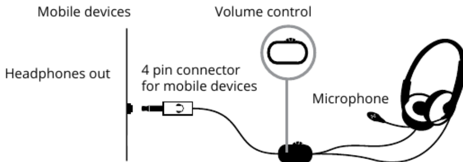
Fig. 1. Connection diagram
